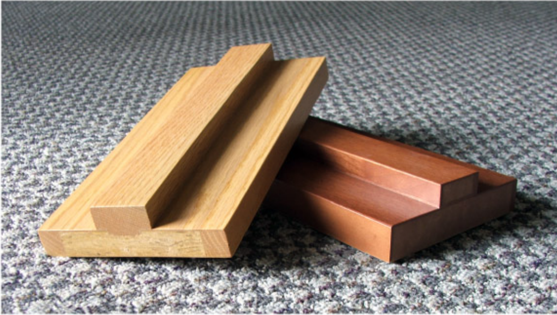
Maiman jamb cross-sections in 20-minute fire-rating (left), and 90-minute fire-rating (right)
