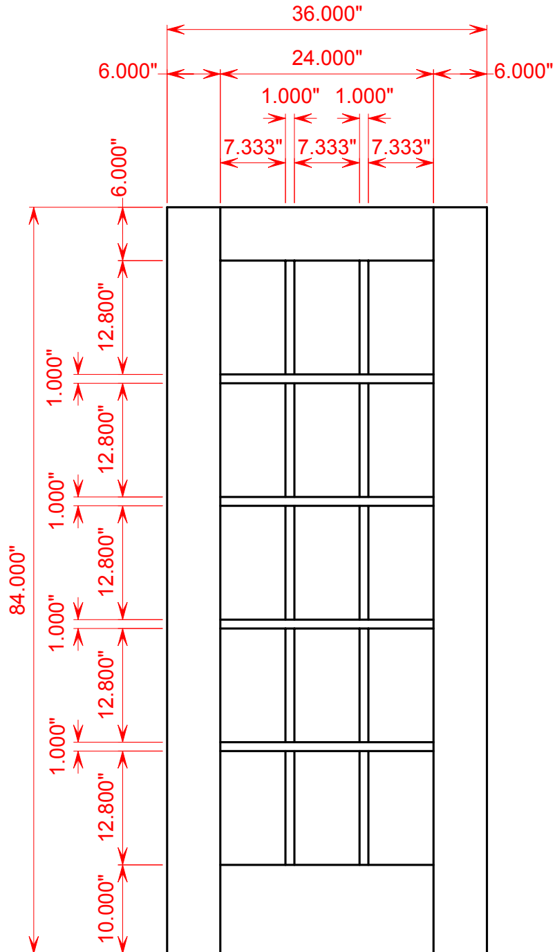
Typical 15 Lite Elevation
