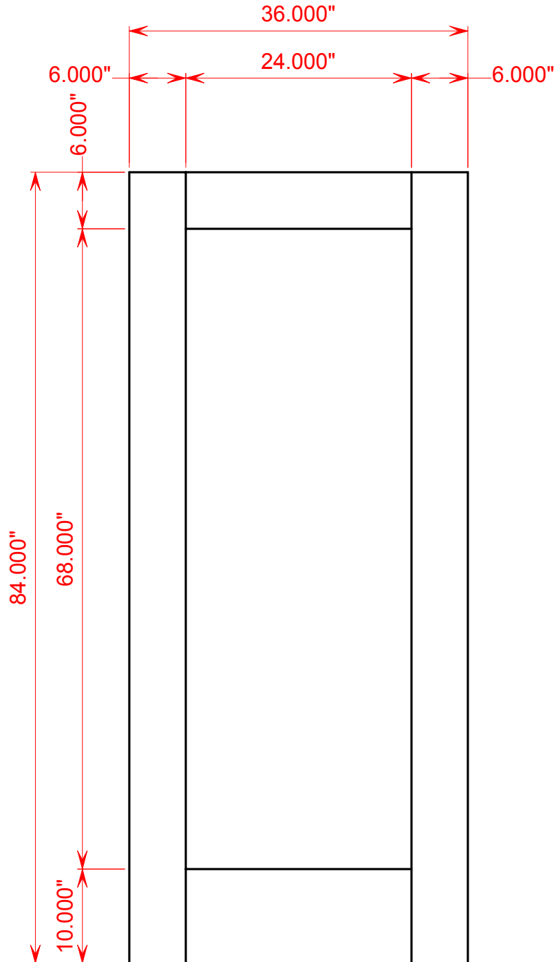
Typical 1 Lite Elevation
